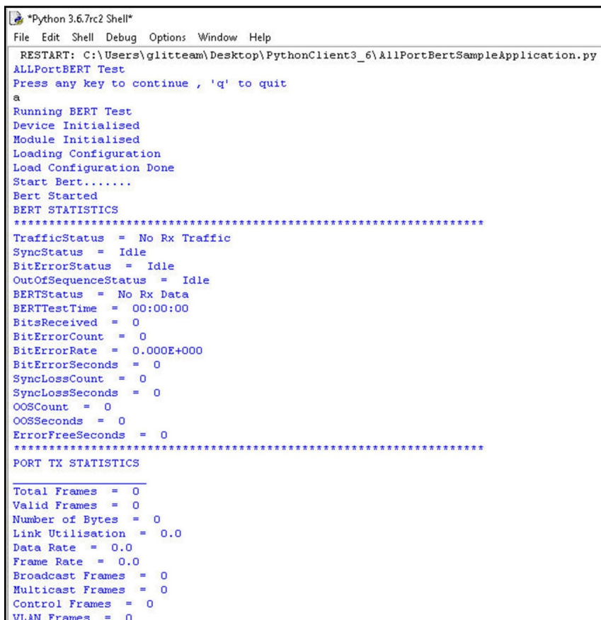
Figure: Sample Python Client Script
