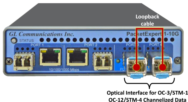
Figure: SonetExpert™ with Optical SFP's Plugged In
