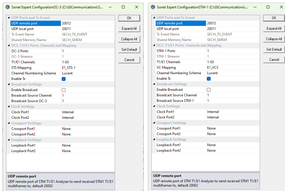
Figure: SEC Configuration Utility for OC-3 and STM-1
