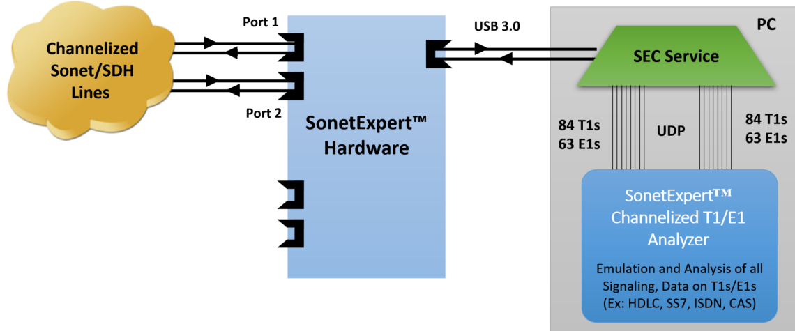
Figure: Architecture of SonetExpert™ Channelized Analyzer
