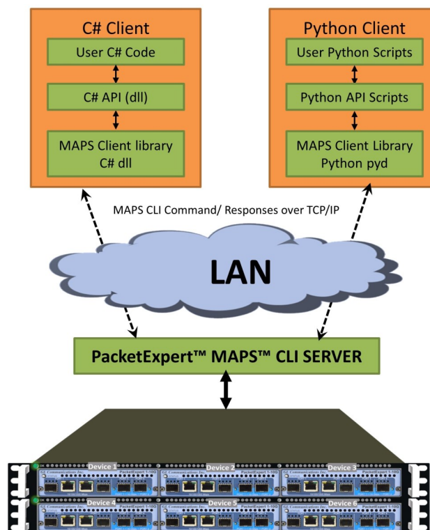
Figure: PacketExpert™ MAPS™ CLI Working Principle
